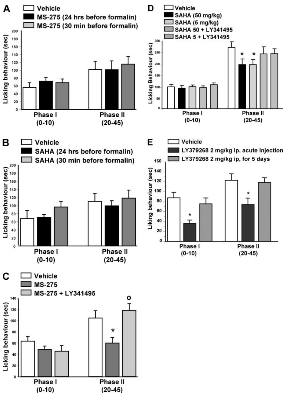
Fig. 2. Repeated systemic injections of MS-275 or SAHA produces analgesia in the second phase of the formalin test in mice. A single injection of MS-275 (3 mg/kg s.c.) (A) or SAHA (50 mg/kg s.c.) (B) either 30 min or 24 h before the injection of formalin in the hind paw did not affect nociceptive behavior. In contrast, a 5-day treatment with MS-275 (3 mg/kg s.c.) (C) or SAHA (5 or 50 mg/kg s.c.) (D) attenuated nociceptive behavior in the second phase of the formalin test. Analgesia was prevented by a single injection of LY341495 (1 mg/kg i.p., administered 30 min before formalin injection) (C and D). Data are means \pm S.E.M. of 12 to 16 mice. *, p < 0.05 (one-way ANOVA + Fisher's PLSD) versus the corresponding group treated with vehicle. \circ , p < 0.05 (one-way ANOVA + Fisher's PLSD) versus the corresponding group treated with MS-275. E, for comparison, the effect of LY 379268 (2 mg/kg i.p.; administered as a single pulse 30 min before formalin or injected daily for 5 days) in the formalin test in mice is shown. Data are means \pm S.E.M. of 8 to 12 mice. *, p < 0.05 (one-way ANOVA + Fisher's PLSD) versus the corresponding group treated with vehicle.
